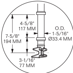
DETAIL B RL shown
