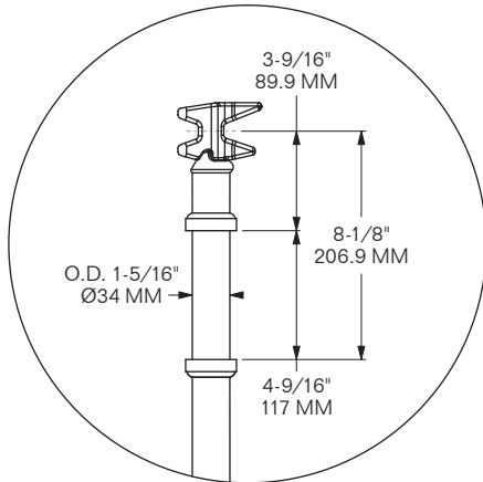
DETAIL A Both ends, LL shown
