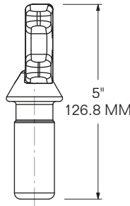
MODEL 1401-2194-L Top Right or Bottom Left
