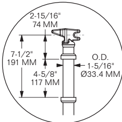
DETAIL A RL shown
